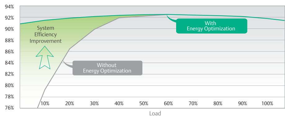
Figure 1: NetSure™ ITM System Efficiency
